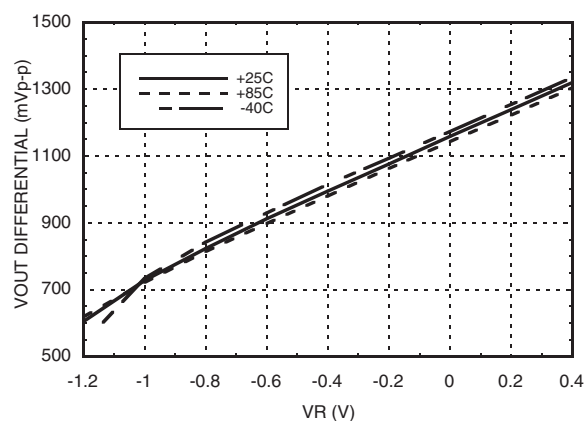
Output Differential Voltage vs. VR [2][3]
